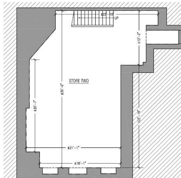
2 FLOOR PLAN - CELLAR LEVEL SCALE: 3/16"=1'-0"
