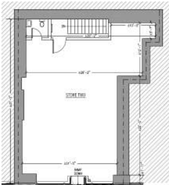
1 FLOOR PLAN - GROUND FLOOR SCALE: 3/16"=1'-0"
